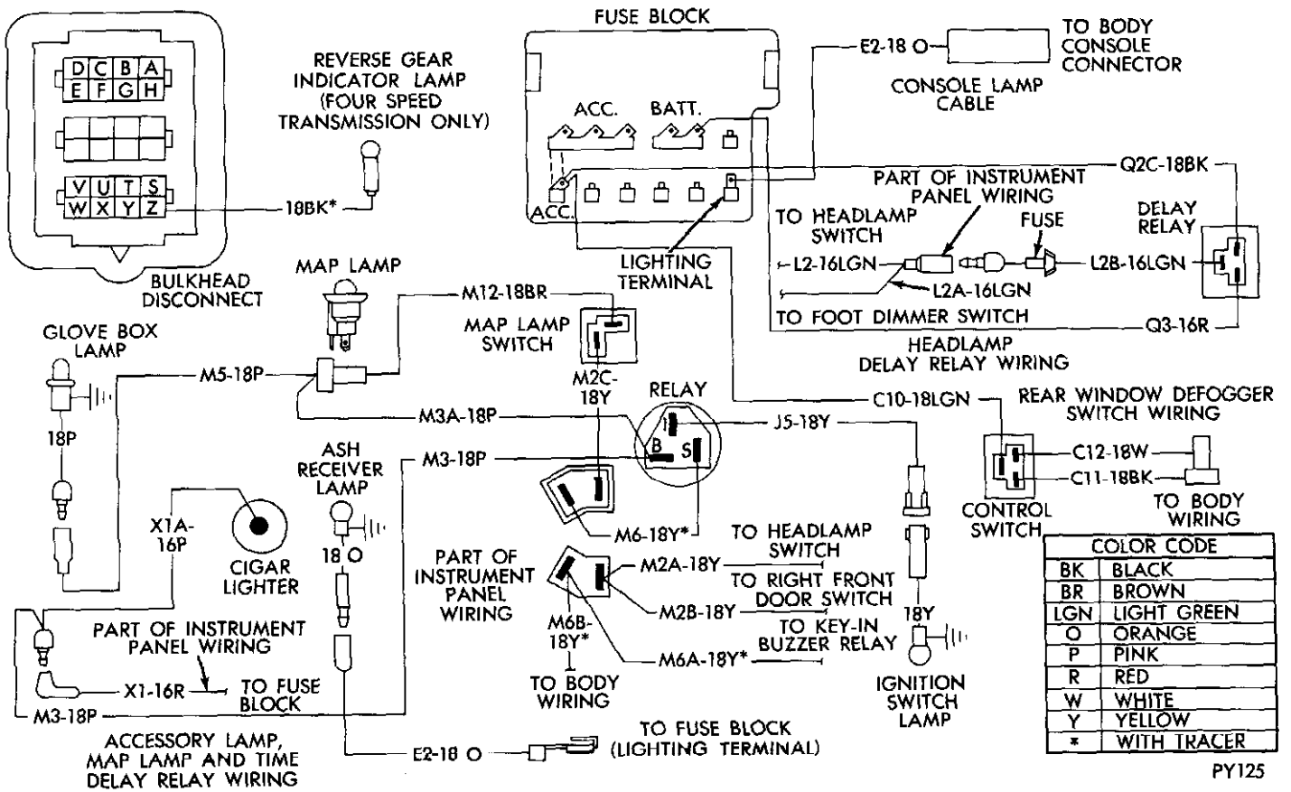
Fig. 24—Instrument Panel Accessory Wiring Diagram—Valiant
