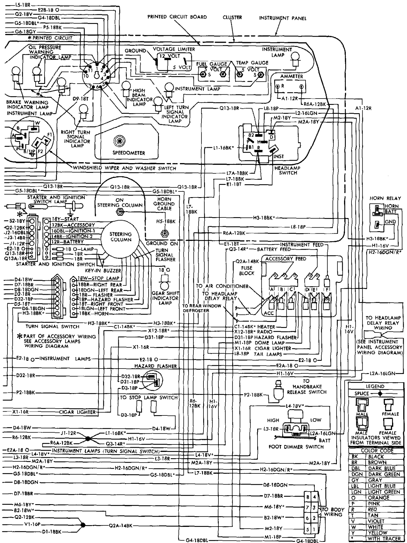
Fig. 23—Instrument Panel Wiring Diagram—Valiant
